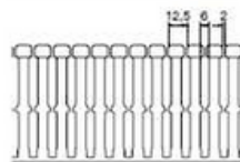
Side Stamping Height 80mm
