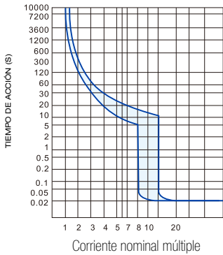
EBS1M -400L
