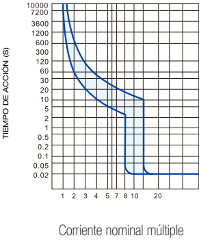
EBS1M -225L
