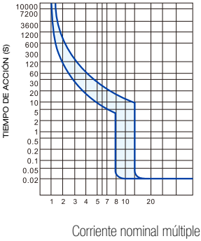
EBS1M -400L
