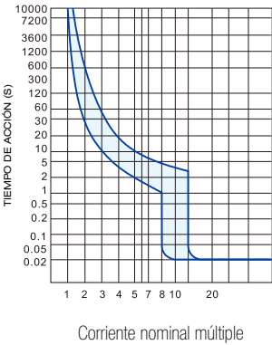
EBS1M -225L
