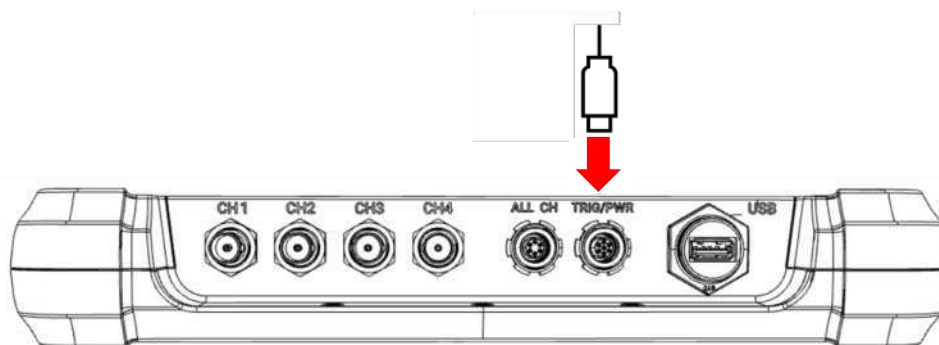
Figure 14 Connect charger
