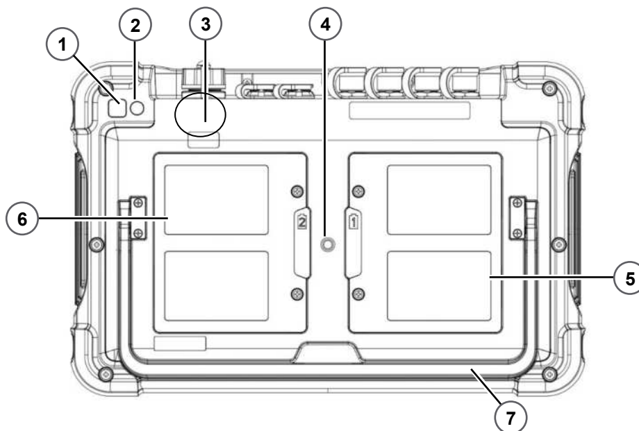
Figure 8 Microlog Analyzer dBX – rear view
