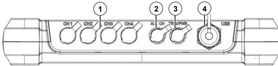
Figure 3 Microlog Analyzer dBX – top view connectors
