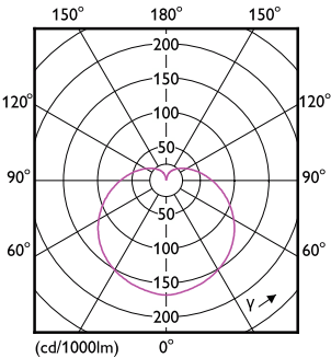
Light Distribution Diagram - CorePro LEDbulb ND 4.9-40W A60 E27 865
