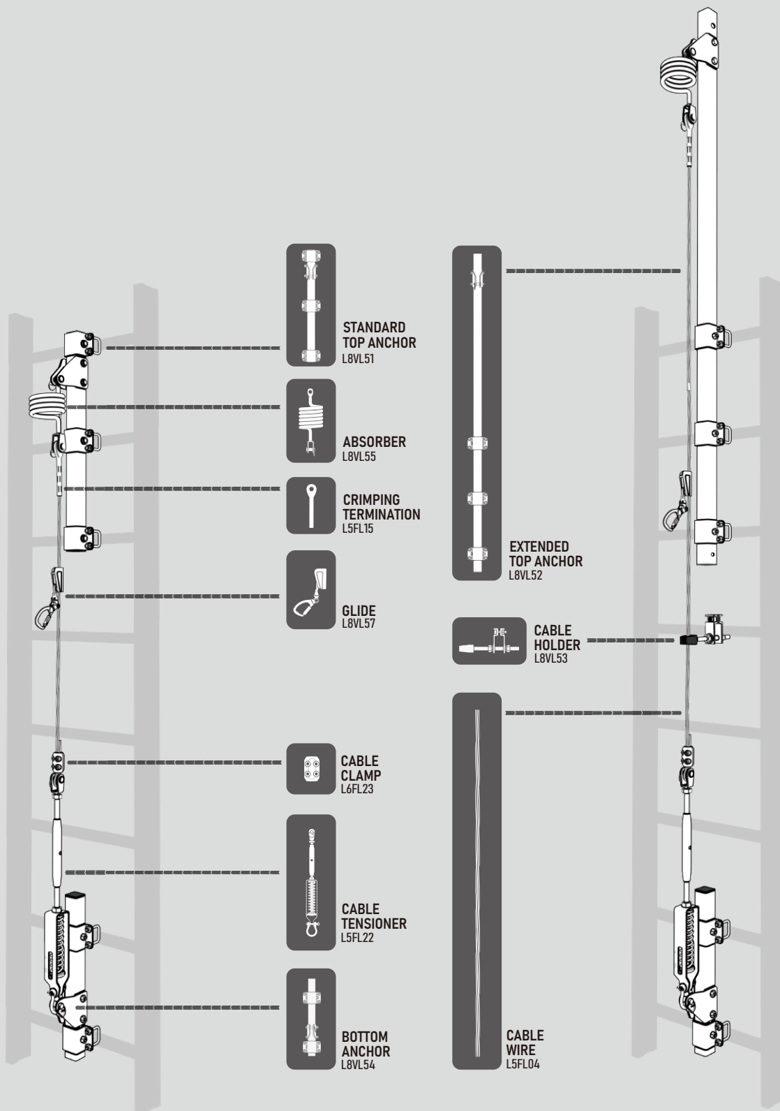
STANDARD MODEL
