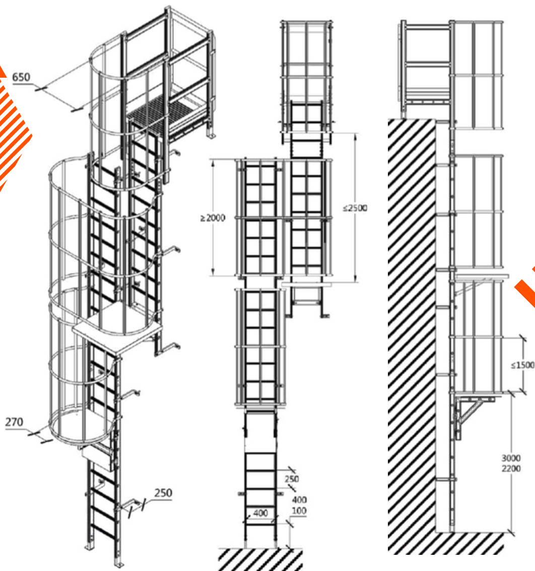
VISTA FRONTAL
